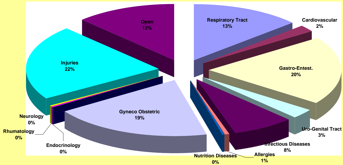
Chak IPD Diagnosis by Category, 2005
